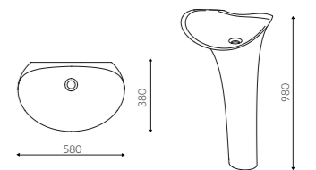
ALICE BACK TO WALL WASHBASIN
