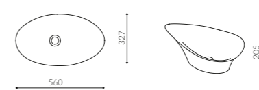
ALICE I COUNTERTOP WASHBASIN
