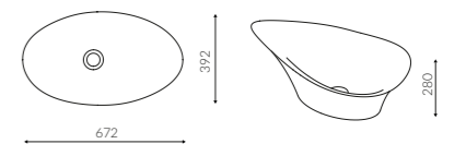
ALICE II COUNTERTOP WASHBASIN
