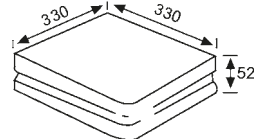
Esquina de peldaño ref. 21 Natural stair-tread corner ref. 21 Cod. 01317
