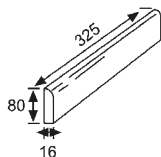
Rodapié 33 Natural skirting board 33 Cod. 01021
