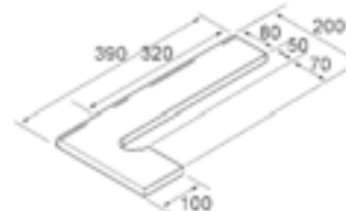
Zanquín ref. 24 izda. Natural string left side ref. 24 Cod. 00034
