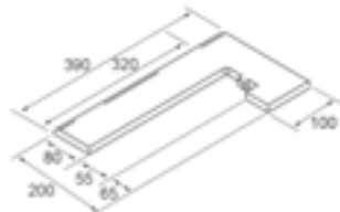
Zanquín ref. 21 dcha. Natural string right side ref. 21 Cod. 01319
