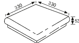
Esquina de peldaño ref. 24 Natural stair-tread corner ref. 24 Cod. 00040
