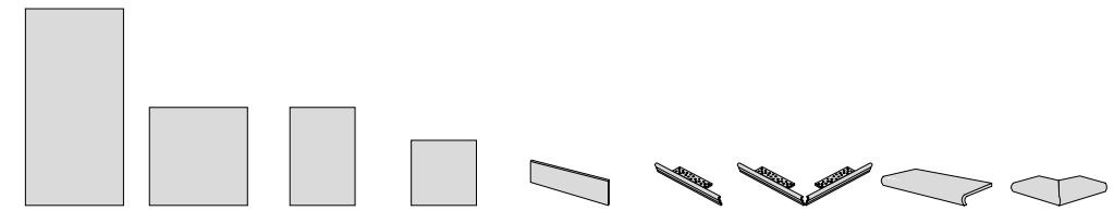
50x100 20"x40" 50x50 20"x20" 33,3x50 13"x20" 33,3x33,3 13"x13" BATTISCOPA 9,5x50 3 7/8"x20" 20 pcs x box TORO 5x33,3 2"x13" 4 pcs x box TORO ANG. 5x33,3 2"x13" 2 pcs x box GRADONE 16,5x30x4,5 6 1/2"x12"x1 7/8" 8 pcs x box GRADONE ANG. 16,5x30x4,5 6 1/2"x12"x1 7/8" 4 pcs x box
