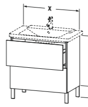
# LC 6600 ↔ 620 mm → P3 Comforts # 233265 # LC 6601 ↔ 820 mm → P3 Comforts # 233285, 233385, 233485 # LC 6602 ↔ 1020 mm → P3 Comforts # 233210, 233310, 233410 # LC 6603 ↔ 1220 mm → P3 Comforts # 233312, 233412 ↗ 481 mm
