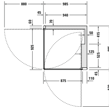
# 770009 00 0 *1 0000, 985 x 885 mm Ecke rechts. Corner right. Rinconera derecha
