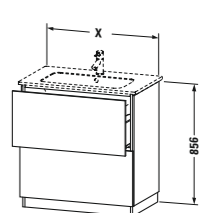
# LC 6681 ↔ 820 mm → ME by Starck # 233683 # LC 6682 ↔ 1020 mm → ME by Starck # 233610 ↗ 481 mm
