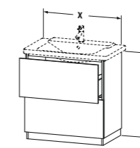
# LC 6612 ↔ 620 mm → P3 Comforts # 233265 # LC 6613 ↔ 820 mm → P3 Comforts # 233285, 233385, 233485 # LC 6614 ↔ 1020 mm → P3 Comforts # 233210, 233310, 233410 # LC 6615 ↔ 1220 mm → P3 Comforts # 233312, 233412 ↗ 481 mm
