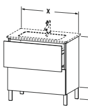
# LC 6626 ↔ 820 mm → ME by Starck # 233683 # LC 6627 ↔ 1020 mm → ME by Starck # 233610 ↗ 481 mm
