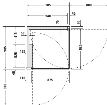
# 770009 00 0 *0 0000, 985 x 885 mm Ecke links. Corner left. Rinconera izq.
