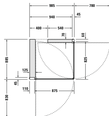
# 770012 00 0 *0 0000, 885 x 885 mm Ecke links. Corner left. Rinconera izq.
