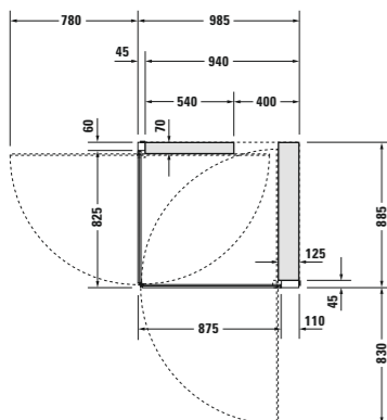
# 770012 00 0 *1 0000, 885 x 885 mm Ecke rechts. Corner right. Rinconera derecha
