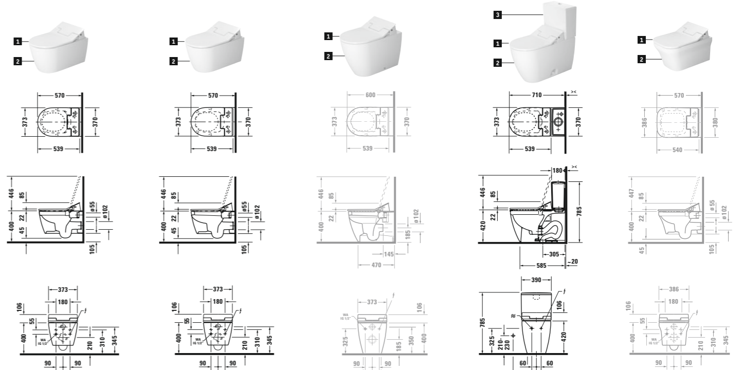
ME by Starck Rimless 1 # 611000 2 # 252959**00 ↗ 4,5 l
