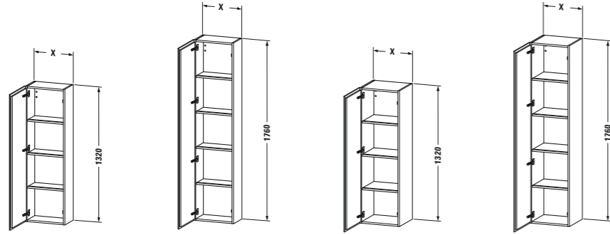
# LC 1168 L/R ↔ 400 mm # LC 1169 L/R ↔ 500 mm ↗ 243 mm
