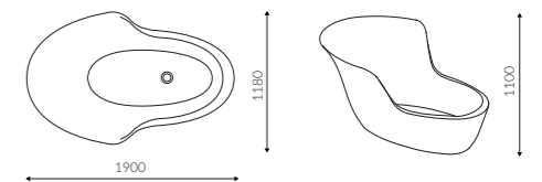
FREE STANDING BATHTUB
