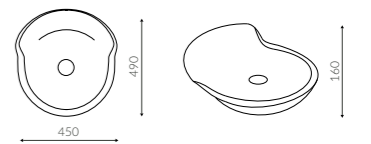
JENA COUNTERTOP WASHBASIN
