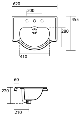
1030 Lavabo incasso 62x46 monoforo (tre fori a richiesta) One hole inset basin 62x46 (three holes on demand)
