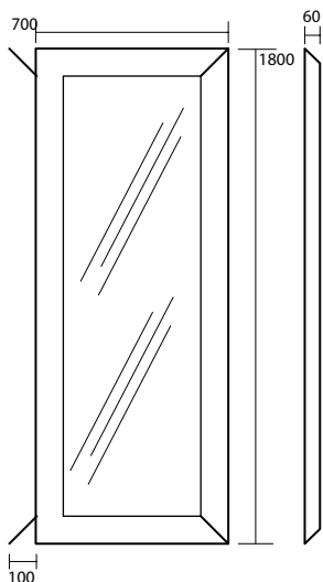
7366 Specchio 70x180 cornice in abete lamellare Mirror 70x180 fir-tree frame
