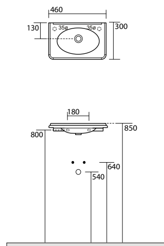
1034 Lavabo 46x30 sospeso (foro rubinetteria dx o sx su richiesta) Wall hung washbasin 46x30 (tap hole on left or right side on demande)
