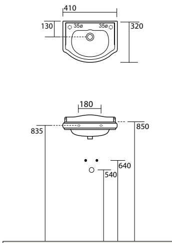
1033 Lavabo 41x32 sospeso (foro rubinetteria dx o sx su richiesta) Wall hung washbasin 41x32 (tap hole on left or right side on demande)
