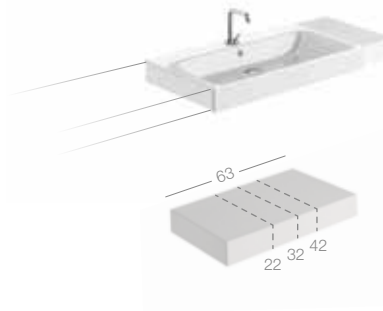
3549 L. 80 X P. 45 lavabo semincasso semi-recessed basic
