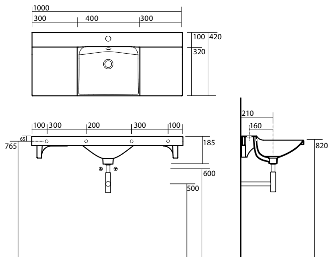
3423 "BUDDY" Lavabo 100x42 sospeso, appoggio monoforo "BUDDY" One hole wall hung or counter top washbasin 100x42
