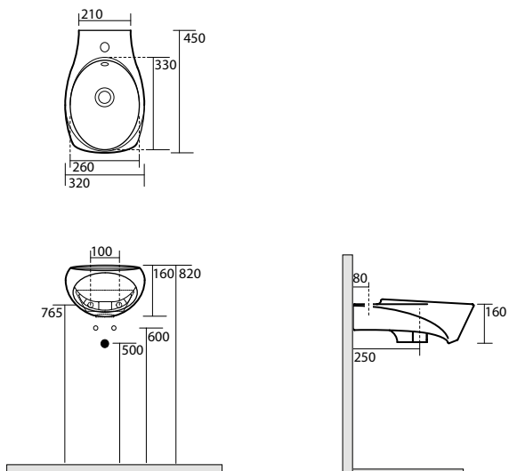
3419 "SHARK" lavabo 32x45 sospeso monoforo "SHARK" one hole wall hung washbasin 32x45
