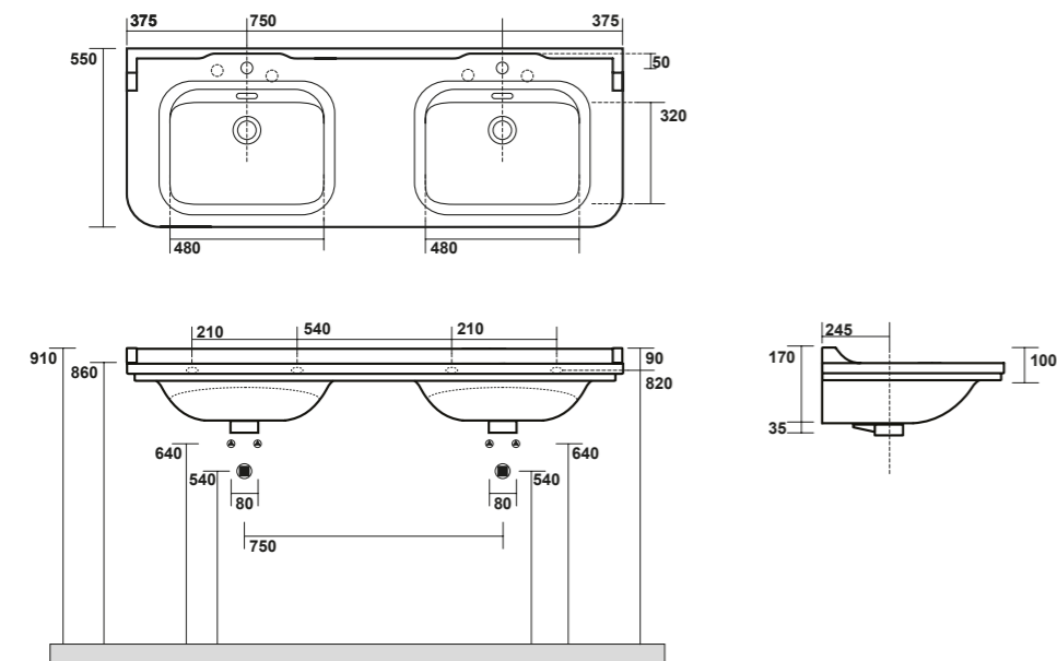
4143 Lavabo 150x55 doppia vasca sospeso monoforo (tre fori a richiesta) One hole wall hung double basin 150x55 (three holes on demand)
