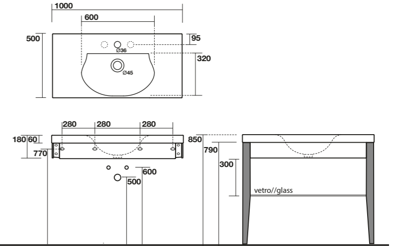
3931 Lavabo cm L.100xP.50 (3 fori a richiesta) Washbasin cm L.100xP.50 (3 holes on demand )
