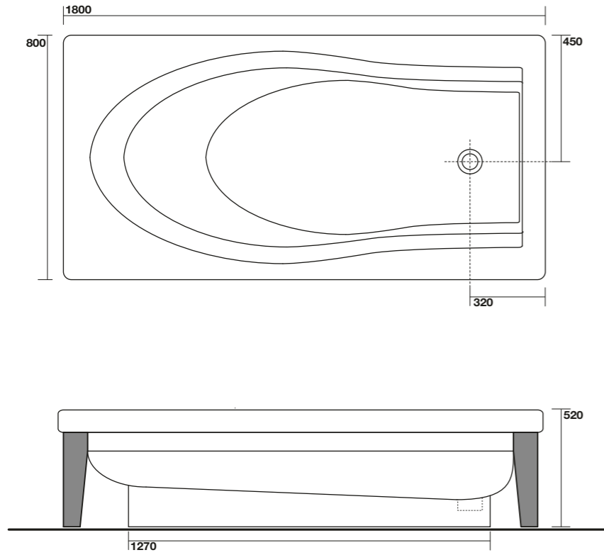
3950 Vasca Bentley cm L.180xP.80xH.52 Bath-tub cm L.180xP.80xH.52
