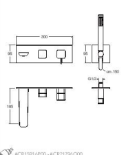
#CR15914P00 - #CR21796C00
