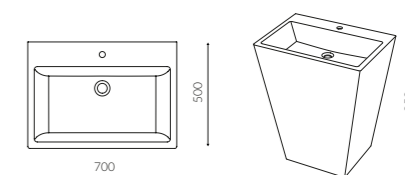
TEBE 700 BACK TO WALL WASHBASIN
