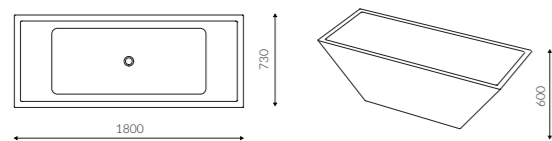
TEBE III FREE STANDING BATHTUB
